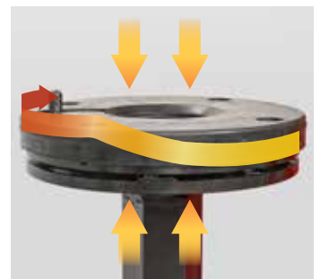
Cam plate rises to exert additional gripping force.
