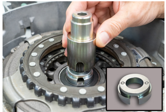
Figure 1: Press-in sleeve in combination with adapter KL-0500-6031
