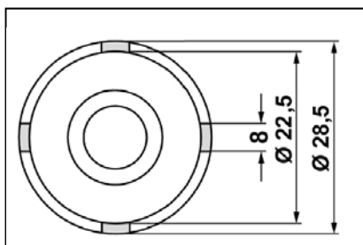
Dimensions KL-0369-601
